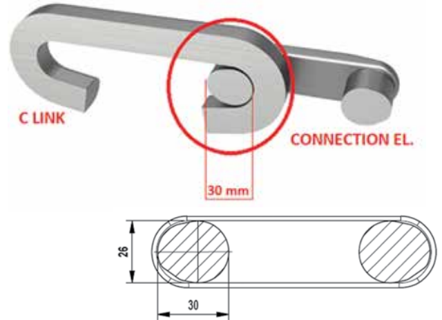
Assembly Hook/Staple
